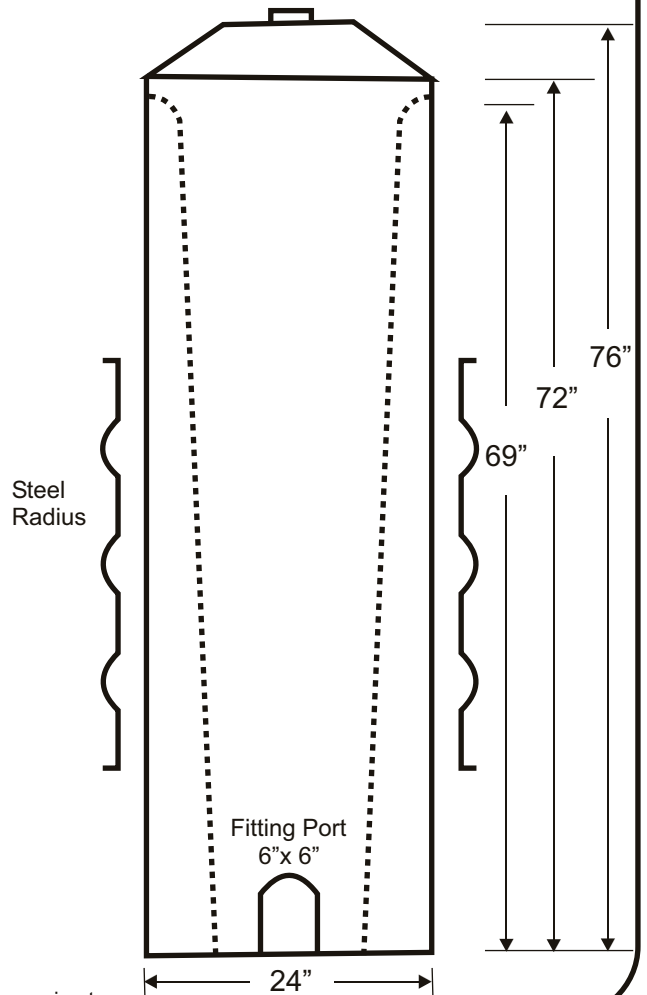
END VIEW
