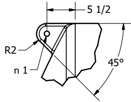
DETAIL B SCALE 1 / 12
